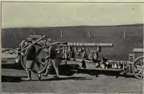
The 4.7-inch Naval Gun from H. M. S. S. Powerful on the march. This gun has a range of nearly eleven miles, throwing ninety-eight pounds of steel and lyddite, and was hauled by a team of thirty-eight oxen. It was attended by a naval contingent from the Powerful .
